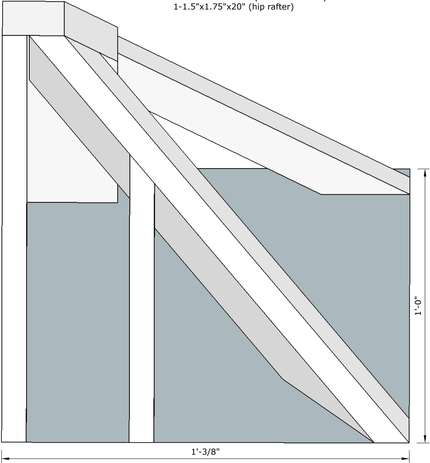
Model 1: 8:12 pitch (33.69°) "Regular pitch, regular plan"
